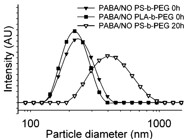
Figure 3. Particle size distributions of undialyzed PABA/NO nanoparticles stabilized by PS- b -PEG (240 nm) (▼) and PLA- b -PEG (225 nm) (■). The slow ripening of undialyzed nanoparticles stabilized by PS- b -PEG shows growth to 440 nm in 20 h (▽).
