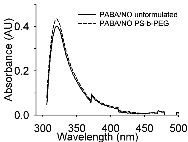
Figure 5. UV-vis absorbance spectra of formulated (stabilized by PS- b -PEG) vs unformulated PABA/NO. The spectra (peak position and intensity) confirm that molecular integrity is preserved during nanoparticle formation and lyophilization.
