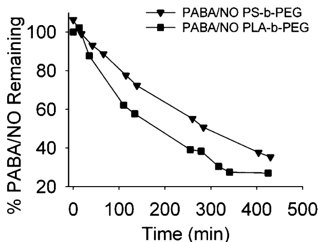
Figure 8. Decomposition of formulated PABA/NO in 4 mM glutathione solution in pH 7.4 phosphate buffer at 25 °C.
