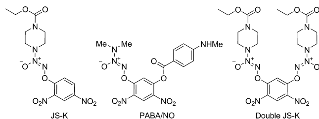
Figure 1. Chemical structures of the diazeniumdiolate nitric oxide prodrugs used in this study.
