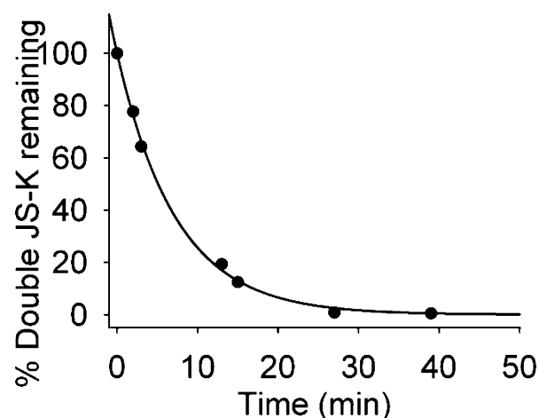
Figure 7. Decomposition of Double JS-K in 4 mM glutathione solution in pH 7.4 phosphate buffer at 25 °C.
