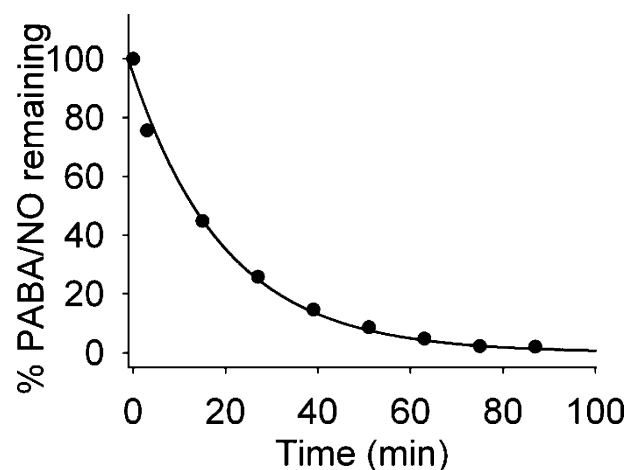
Figure 6. Decomposition of PABA/NO in 4 mM glutathione solution in pH 7.4 phosphate buffer at 25 °C.
