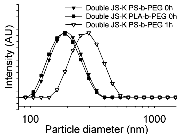
Figure 4. Particle size distributions of undialyzed Double JS-K nanoparticles stabilized by PS- b -PEG (200 nm) (▼) and PLA- b -PEG (195 nm) (■). The growth of the PS- b -PEG stabilized particles (to 290 nm) over 1 h is shown (▽).
