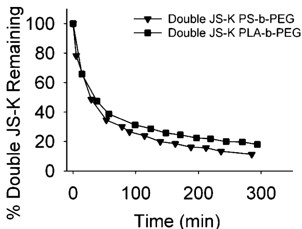
Figure 9. Decomposition of formulated Double JS-K in 4 mM glutathione solution in pH 7.4 phosphate buffer at 25 °C.
